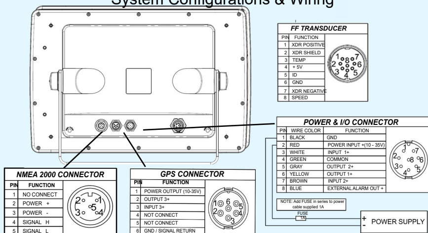
System Configurations & Wiring
